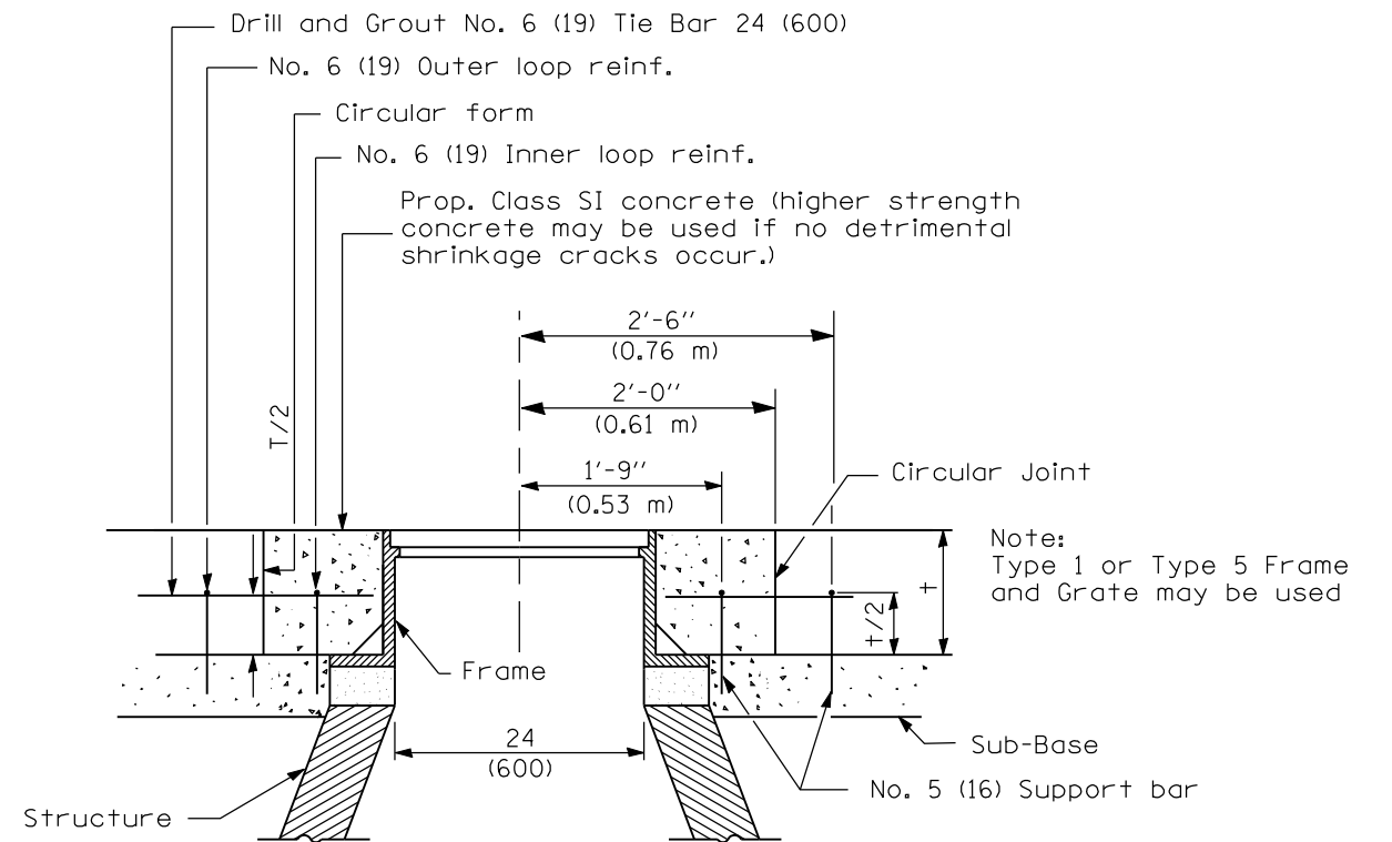
DETAIL OF REINFORCEMENT FOR PAVEMENT ROUNDOUT
