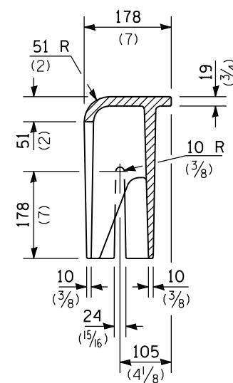
SECTION E-E
