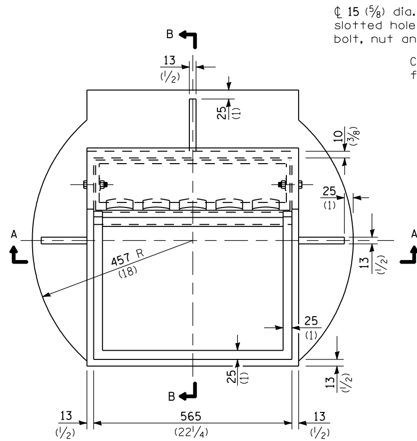
CAST FRAME
