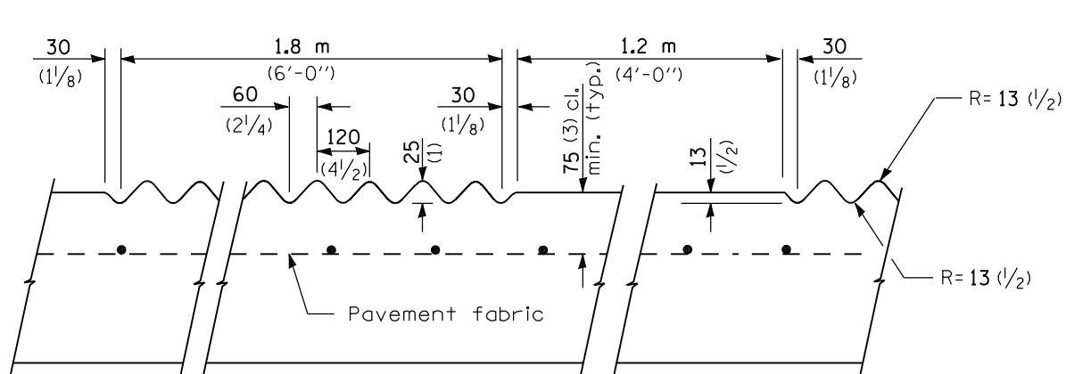
SECTION B-B
