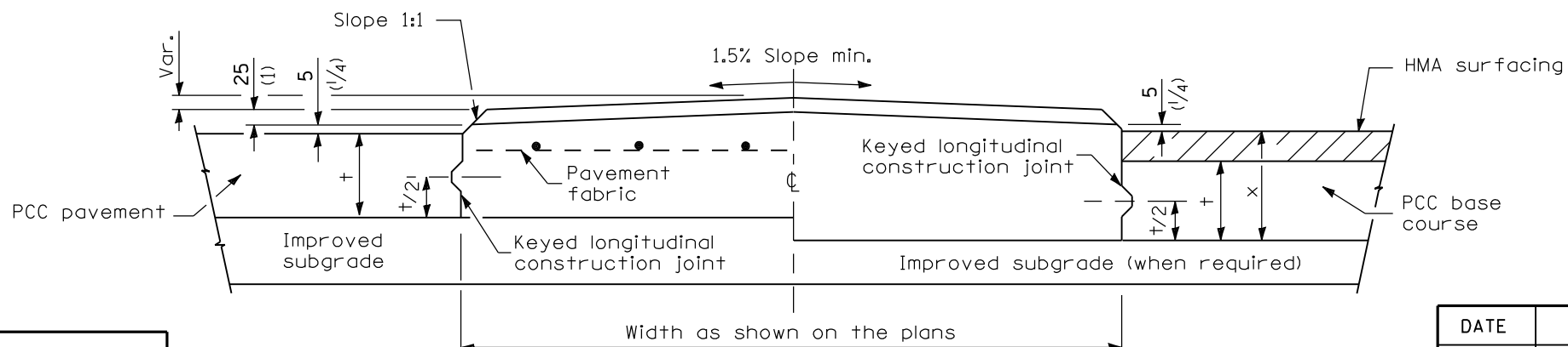
HALF SECTION FOR PCC PAVEMENT
