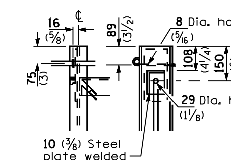
DETAIL P
