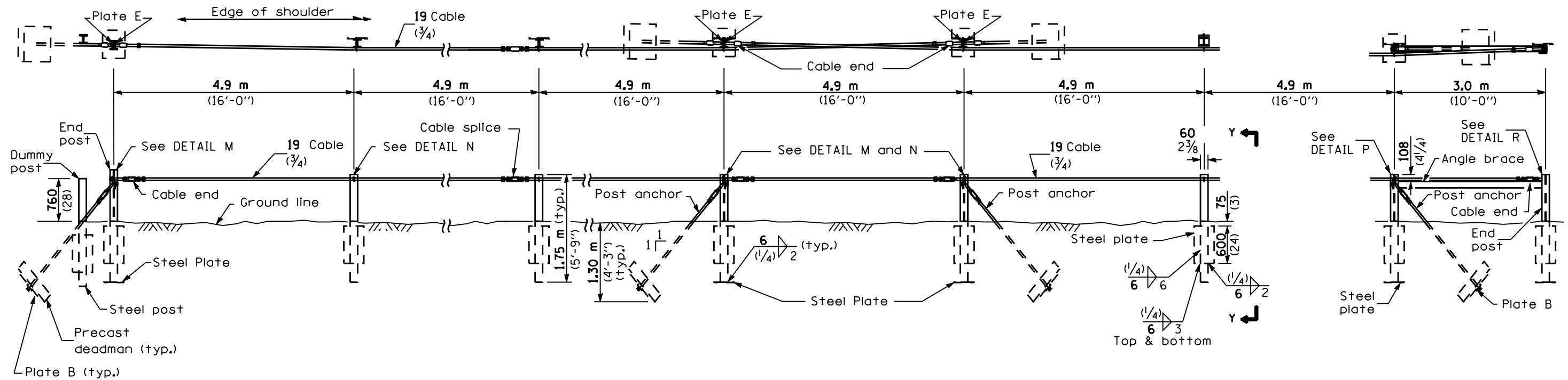
INTERMEDIATE ANCHOR ARRANGEMENT
