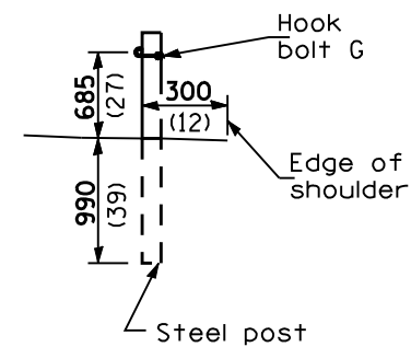
VIEW Y-Y
