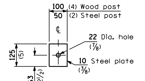
PLATE D
