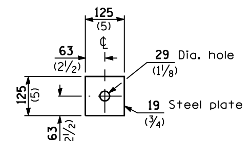
PLATE B
