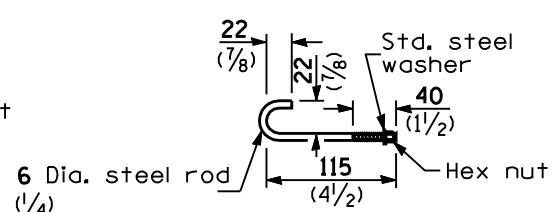
HOOK BOLT G
