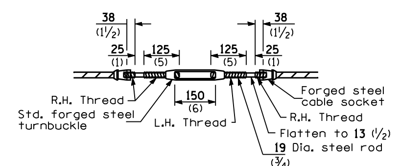
CABLE SPLICE
