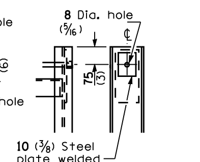
DETAIL R
