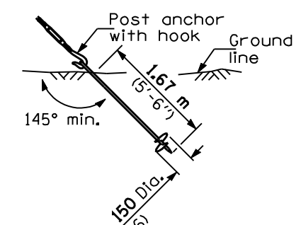
STEEL SCREW
