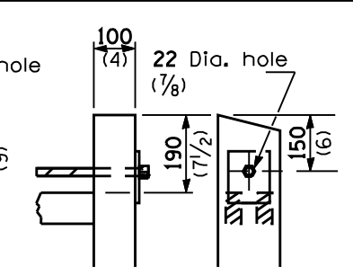
DETAIL L
