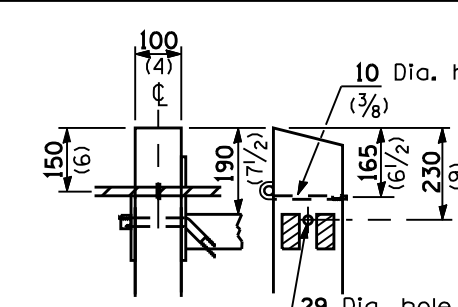
DETAIL K
