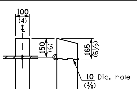
DETAIL J
