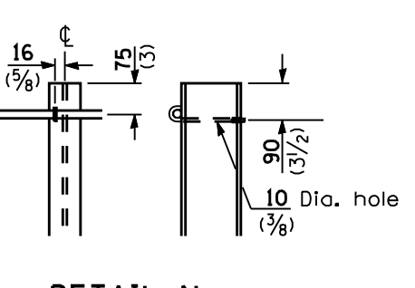
DETAIL N
