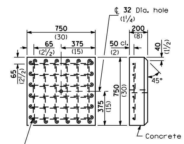
PRECAST DEADMAN
