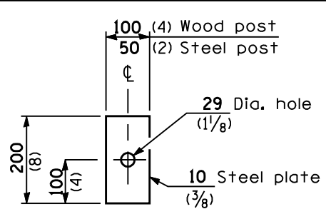
PLATE C
