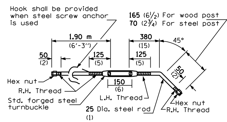
POST ANCHOR
