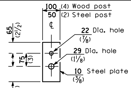
PLATE E
