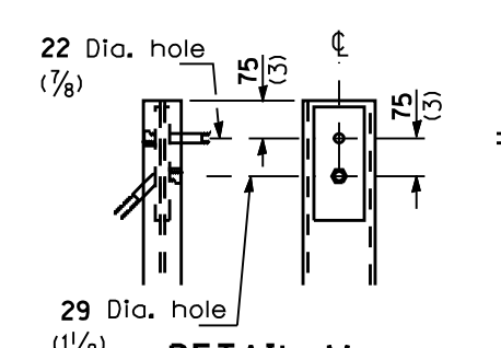
DETAIL M
