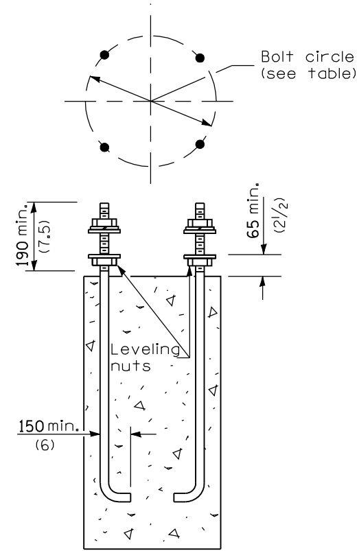
ANCHOR ROD DETAIL
