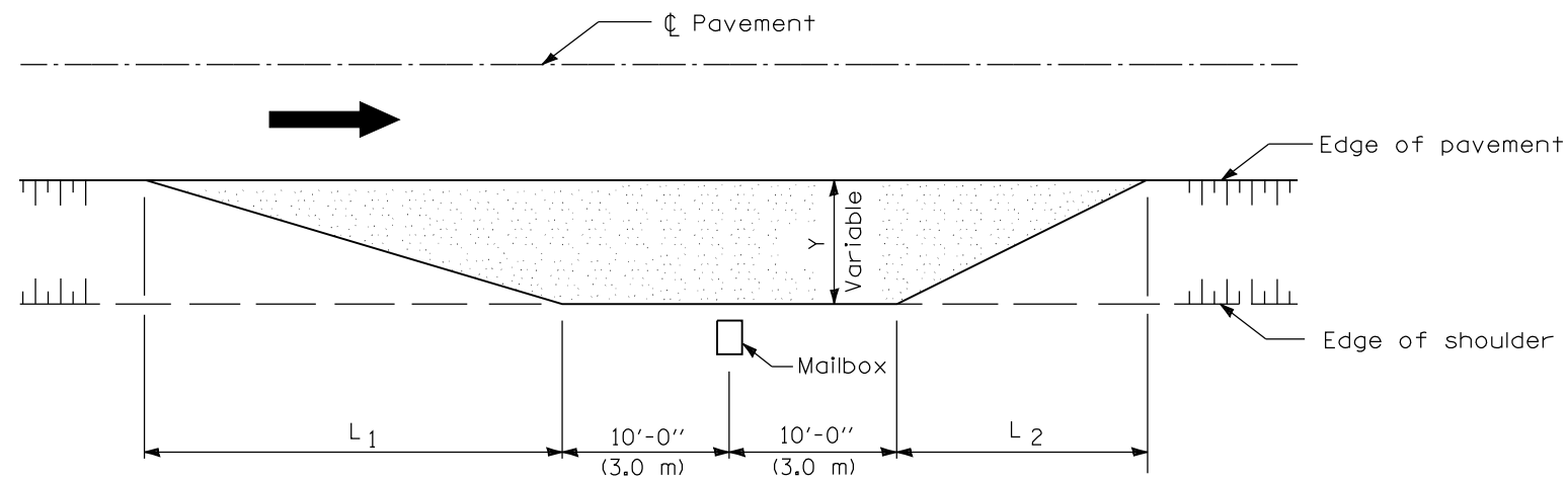
TYPICAL APPLICATION
