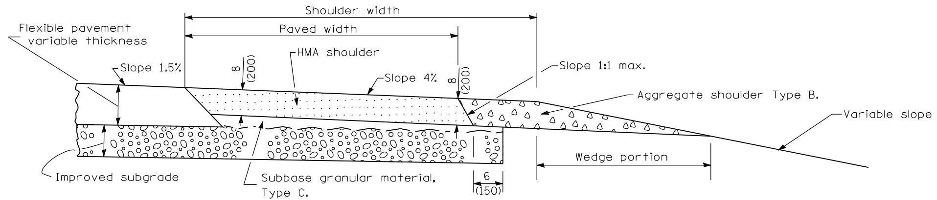
SHOULDER FOR TANGENT PAVEMENT
