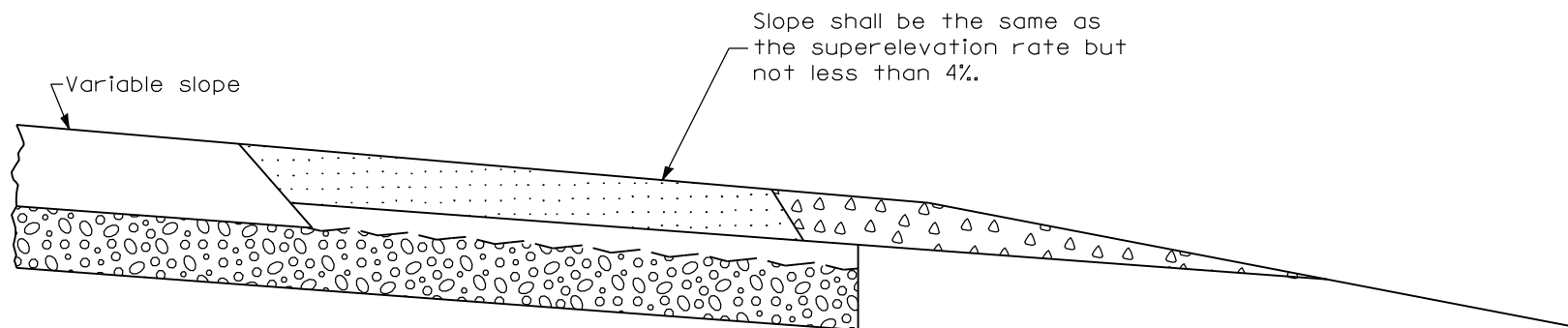
SHOULDER FOR SUPERELEVATED PAVEMENT (INSIDE OF CURVE)
