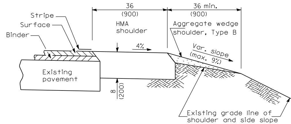
HMA SHOULDER AND AGGREGATE WEDGE WITH RESURFACING (Cross-section G)
