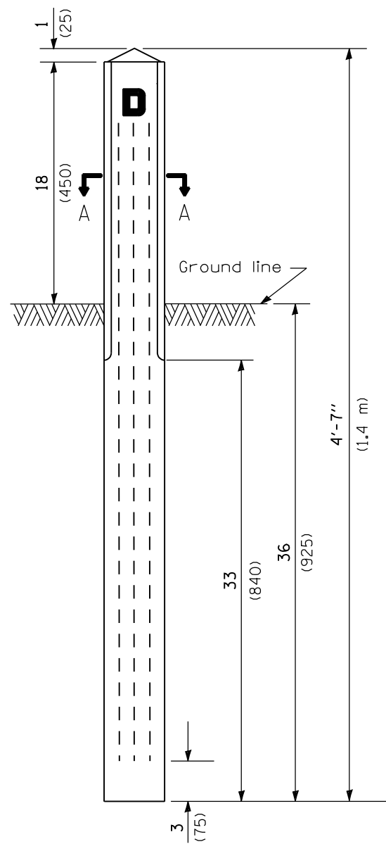
FRONT ELEVATION
