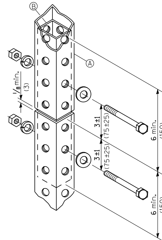
SPLICE DETAIL
