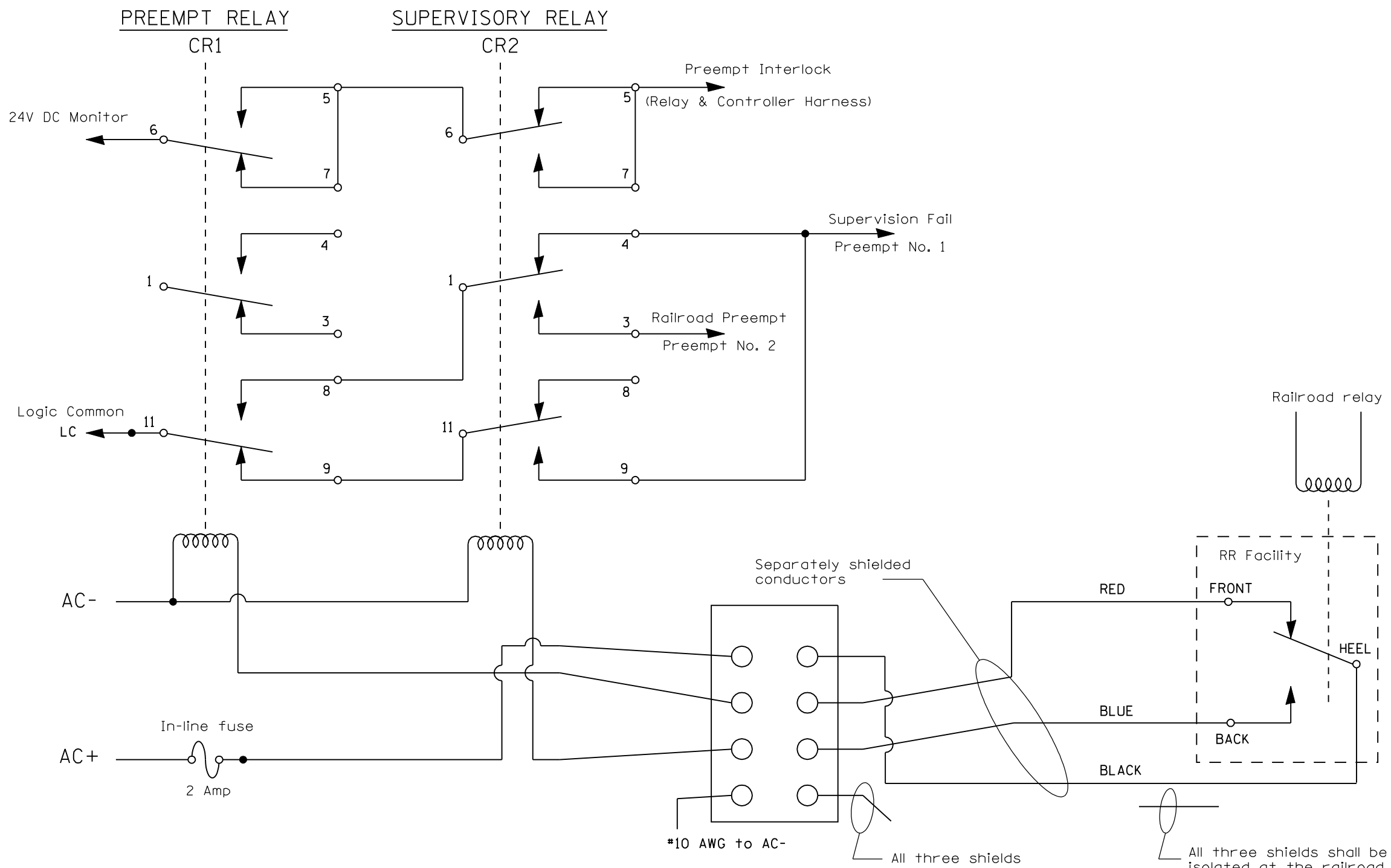
RELAYS IN NON-PREEMPT STATE - RAILROAD AND PREEMPT RELAYS ENERGIZED
