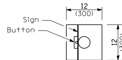
TOP VIEW TYPICAL ONE BUTTON
