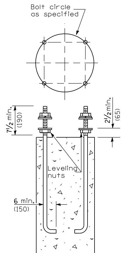
ANCHOR ROD DETAIL
