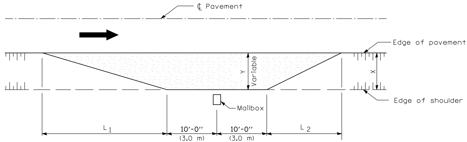
TYPICAL APPLICATION
